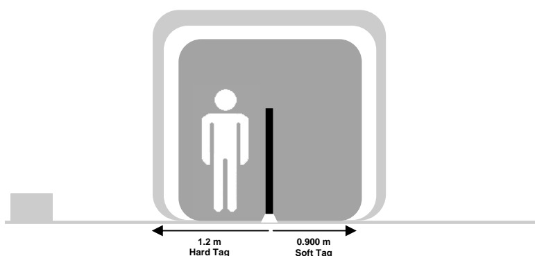
MAXIMUM DETECTION DISTANCES WITH TAG DEPENDING ON ENVIRONMENT
